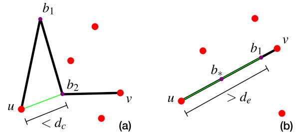
Fig. 7: Flexible edges contraction and expansion. (a) Contraction. Since b_1 previous bend ( u ) and following bend ( b_2 ) are closer than d_c and no nodes are in the triangle \Delta ub_1 b_2 , the bend b_1 and its incident segments are substituted by the green segment. (b) Expansion. Since the first edge segment is longer than d_e , a new bend b_* is introduced and the segment is substituted by the two green ones.
