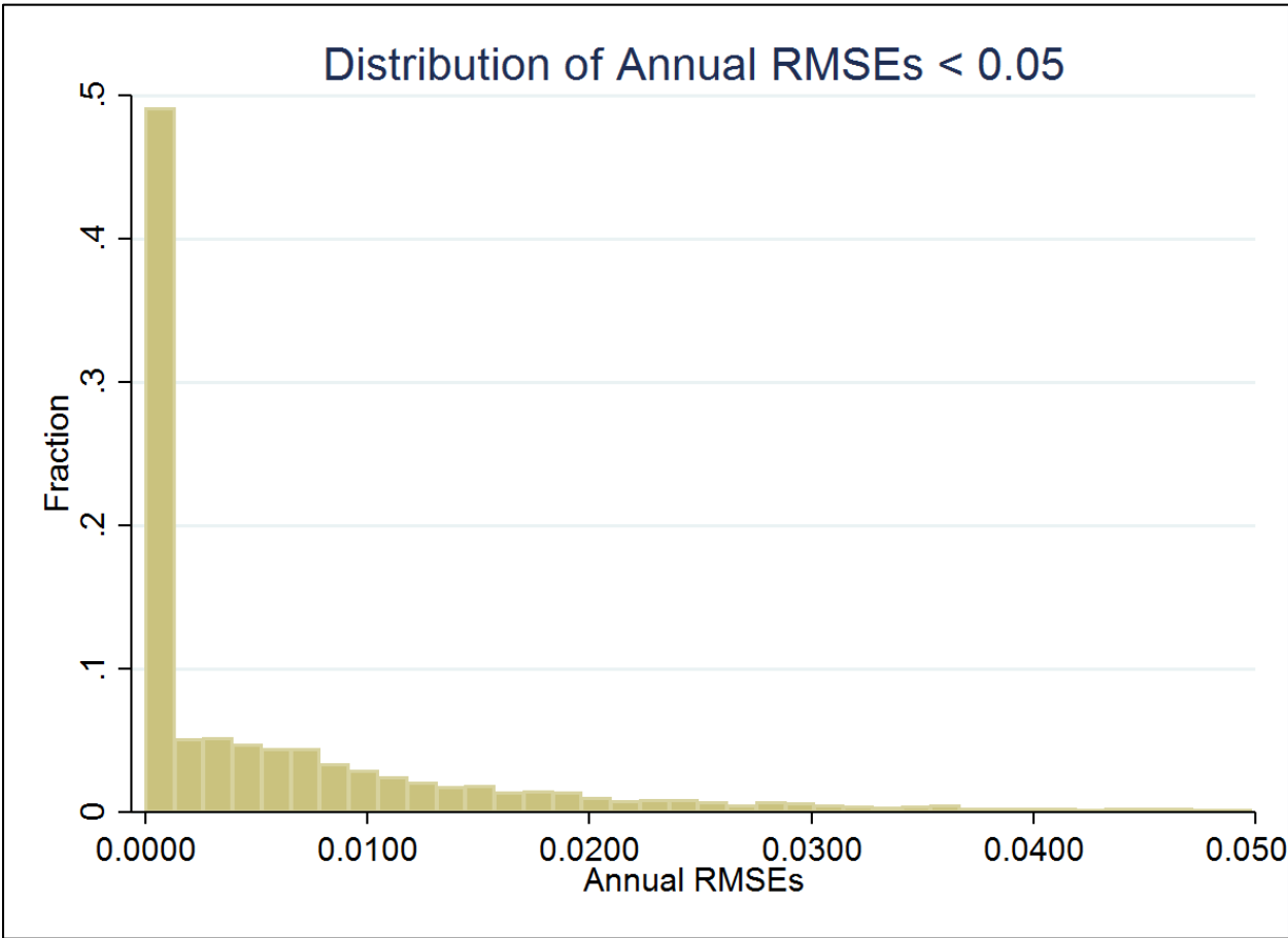
Figure 1. The distribution of annual RMSEs (CHF as numeraire)
