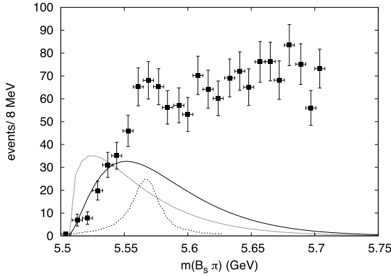
Fig. 1. D\bar{0} data (points), extracted resonance signal (dashed line), and threshold models.
