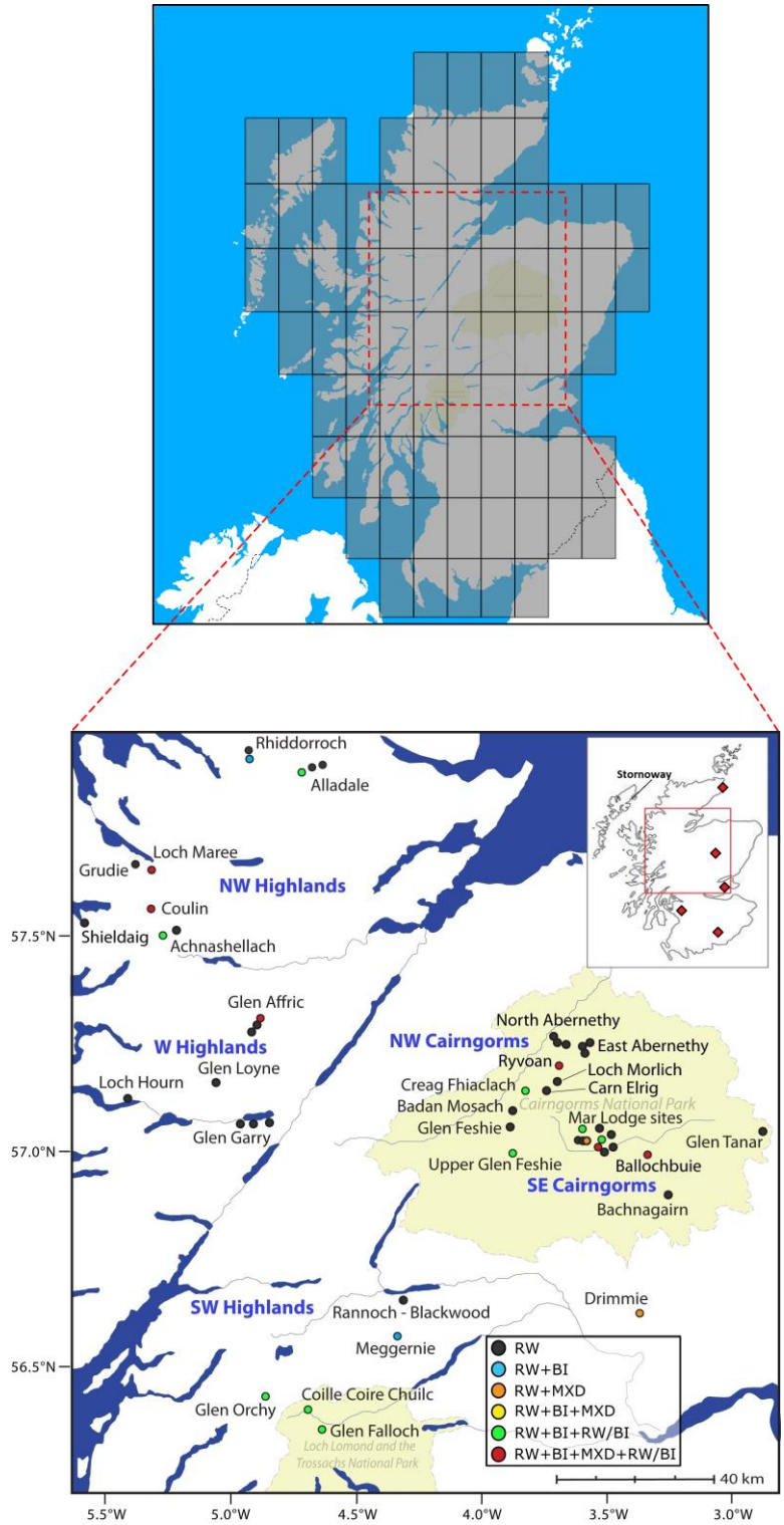
Figure 1: Map of Scotland and location of field containing 76 individual 0.5° reconstruction grids along with the location of RW, BI, MXD and composite BI/RW site chronologies used for spatial reconstruction. (Approximate locations of instrumental records included in the SMT temperature series are marked in the inset map.)
