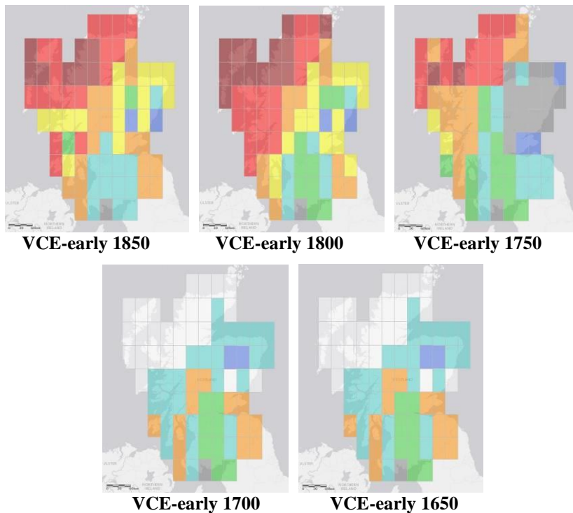
Figure 5: Independent verification CE (VCE) for the (a) late (1877-2006) and (b) early (1872-1900) period with reconstruction nests in 50 year intervals. Reconstructions are based on RW (SF, pre/post-CID) + BI - composite chronologies & separate MXD chronologies. (White grids signify no available data for a specific period. Grey grids represent VCE ≤ 0.)
