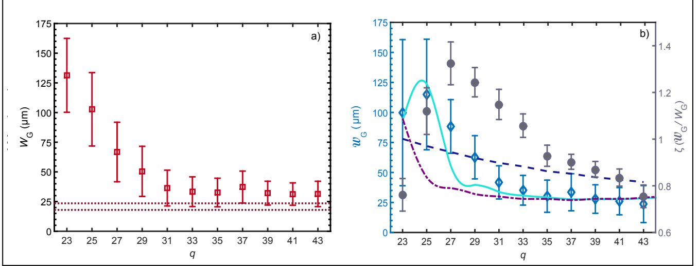
Figure 3. a) Harmonic source intensity width W_G plotted as a function of order (open red squares). The brown dotted lines bound an interval consistent with equation 20 and the SFA calculation. b) Harmonic source coherence width w_G plotted as a function of order (open blue diamonds). The three lines corresponds to fits derived from equation 8 with C'(\Delta\phi_0, \chi_0) = 0 and: no dipole phase but a partially coherent driver (dashed navy blue line), dipole phase with a fully coherent driver (dot-dashed purple line) or the full expression — dipole phase + partially coherent driver (solid light blue line). The normalised coherence width ( \zeta ) is plotted with filled grey circles, these values are identical to those plotted in figure 2 by virtue of the properties of the Gaussian-Schell model.
