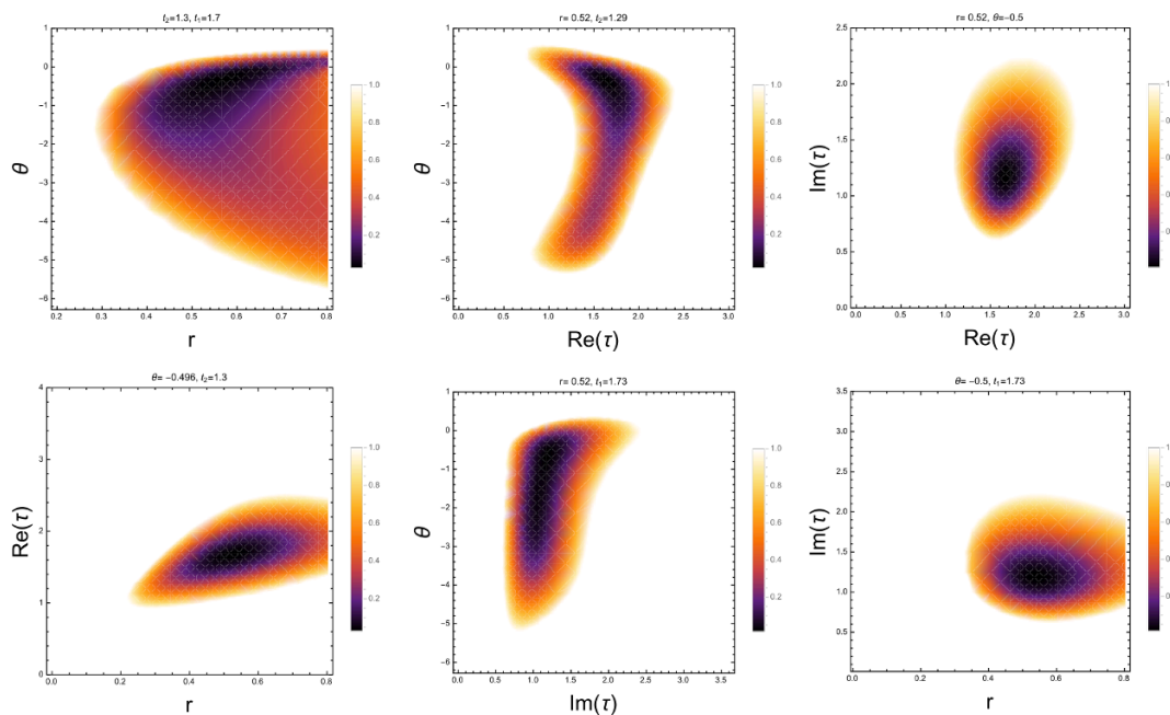
Figure 10. Density plot for \epsilon for a configuration of non-zero fluxes F_1 = 2, F_2 = 2, F_3 = 1, F_4 = 3, H_1 = 4, H_2 = 4, H_3 = 2 and H_4 = 1 . The CS modulus is in the conifold patch z_C = r e^{i\theta} and evaluations are performed to order 200 in the period series expansion \Pi_C . The projections on the different planes are made by fixing the values of the moduli at r = 0.52, t_1 = 1.73, \theta = -0.496, t_2 = 1.295 respectively. For this configuration, there is a dS vacuum approximately at r = 0.63, t_1 = 1.55, \theta = -0.03, t_2 = 1.25 . The smallest values of \epsilon in these regions are \epsilon \sim 0.03 . A sample \eta eigenvalue is \eta_{50} = -0.011 , the subindex denotes that \eta is computed at order 50, corresponding to the eigenvector \eta_{\min} \sim (0.67, -0.71, -0.096, -0.22) , giving as the preferential inflationary directions along t_1 and t_2 . For the canonically normalized fields the displacements in Planck units, in the represented region, are of order \Delta\phi_r \sim 0.124M_{\text{Pl}}, \Delta\phi_\theta \sim 0.58M_{\text{Pl}}, \Delta\phi_{t_2} \sim 0.69M_{\text{Pl}}, \Delta\phi_{t_1} \sim 0.65M_{\text{Pl}} .
