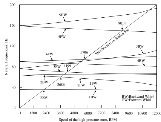
Figure 12. Campbell diagram of updated DSM critical speeds excited by HP rotor.
