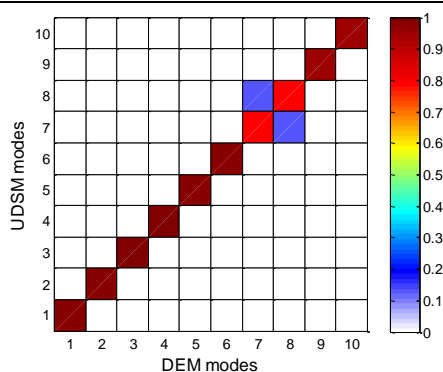
Figure 9. MAC comparison of the updated scaled DSM with the DEM.
