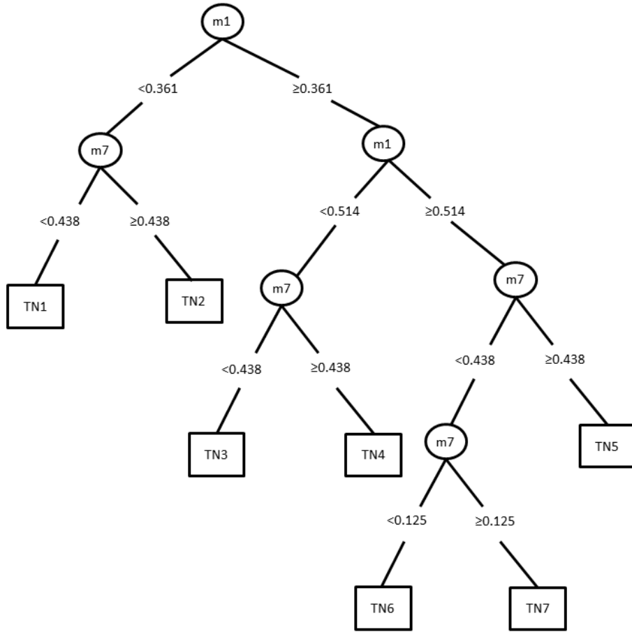
Figure 4: Constructed tree by CART on Energy Efficiency Heating example. Boxes represent the terminal leaf nodes with labels inside, while circles represent other nodes, where the symbol inside refers to the feature where the split takes place. The splitting rules are given on the corresponding paths.
