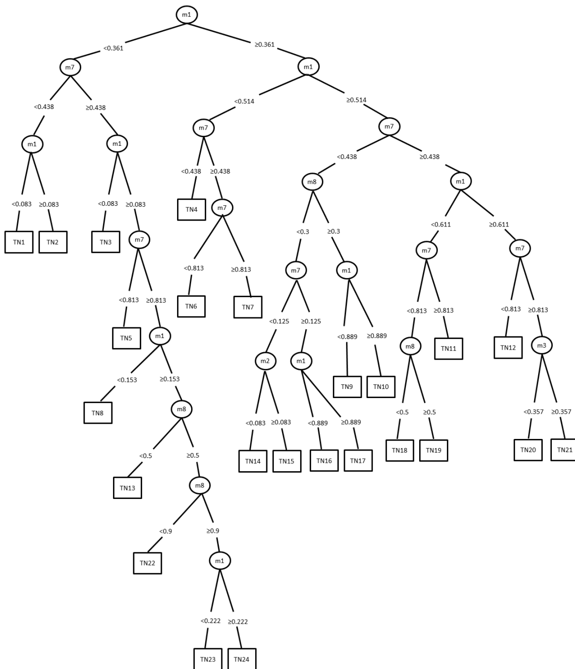
Figure 5: Constructed tree by M5' on Energy Efficiency Heating example. Boxes represent the terminal leaf nodes with labels inside, while circles represent other nodes, where the symbol inside refers to the feature where the split takes place. The splitting rules are given on the corresponding paths.
