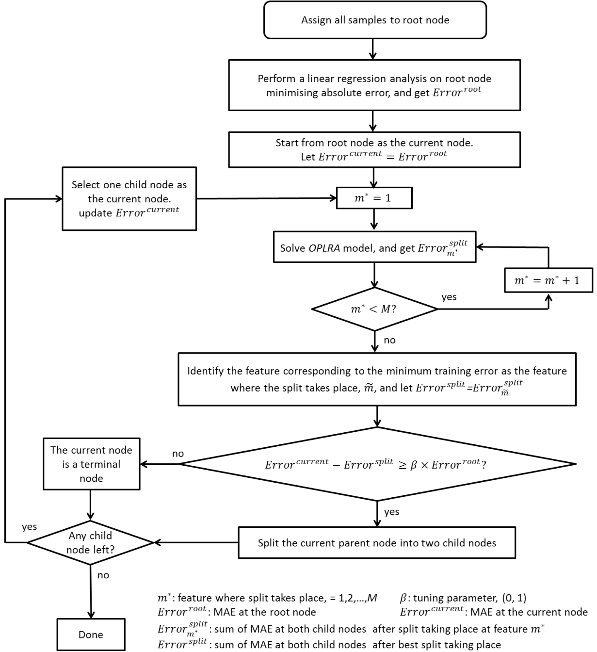
Figure 1: Flowchart of the proposed regression tree approach.
