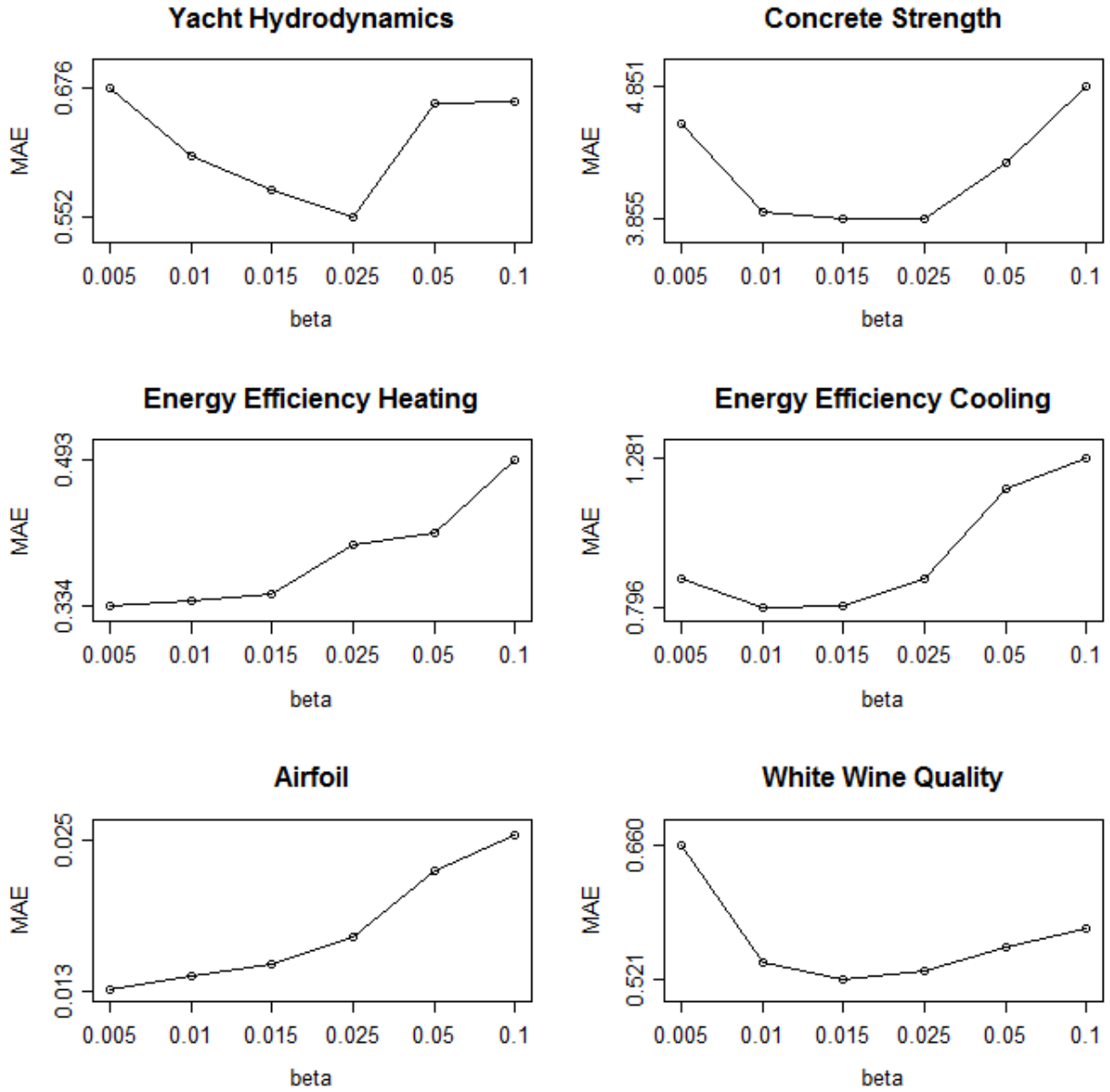
Figure 2: Sensitivity analysis for \beta of all data sets.
