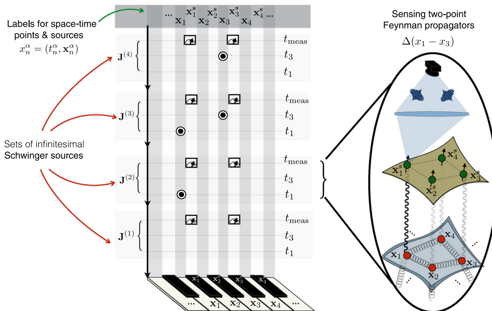
FIG. 2. Schematic representation of the quantum sensing for Feynman propagators. The different indexes for the lattice sites \mathbf{x} \in \Lambda_s , as well as the corresponding \mathbb{Z}_2 sensors labeled by \mathbf{x}^s , are mapped onto the keys of a piano. The set of pulse sequences \mathbf{J}^{(m)} that couple the sensors to the field Eq. (14) corresponds to a piano score that indicates the sequence of keys (sensors) that must be pressed (coupled to the field) at different instants of time to produce a melody (spin-parity measurement) that encodes the relevant information about the Feynman propagators.
