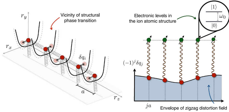
FIG. 3. Effective \lambda\phi^4 QFT for ion crystals and quantum sensing scheme. Left: In the vicinity of the linear-to-zigzag structural phase transition of a trapped-ion crystal, the transverse zigzag vibrations yield the soft mode that contains the universal properties of the transition. Right: The slowly varying envelope of the zigzag distortion Eq. (32) allows us to develop a gradient expansion that leads to the effective \lambda\phi^4 QFT. By exploiting two electronic levels of the ions, and a state-dependent dipole force Eq. (49), one can infer the generating functional of the QFT.
