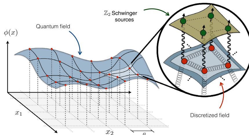
FIG. 1. Schematic representation of the Schwinger sensors for the generating functional. We represent a quantum scalar field \phi(x) in a D = 2 + 1 space-time, which is discretized into a d = 2 spatial lattice, while letting the time coordinate continuous. Inset: Zoom of a small space region, where the field at each point (red circles) is coupled to the fields at neighboring points (small springs) and can be excited by its coupling (wavy lines) to generalized quantum-mechanical Schwinger sources (green circles with arrows). These \mathbb{Z}_2 Schwinger sources will also function as quantum sensors for the generating functional.
