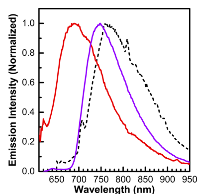
Figure 3. Normalized emission spectra recorded upon visible-light excitation of 5 mM solutions of 1 (dashed black, \lambda_{\text{ex}} 470 nm), 2 (red, \lambda_{\text{ex}} 475 nm), and 3 (purple, \lambda_{\text{ex}} 465 nm) in 4:1 ethanol/methanol at 77 K. Complications in baseline correction by optical interference from bubbles generated by boiling nitrogen surrounding the NMR tube used to record the spectra are depicted in Figures S2–S4 in the SI.
