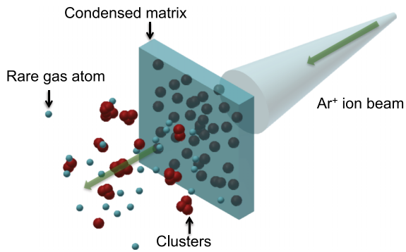
FIG. 1. Schematic diagram of the concept of the Matrix Assembly Cluster Source (MACS). The matrix is formed by evaporation of atoms of cluster material (e.g., Ag or Au) and rare gas atoms (e.g., Ar) condensed at the same time onto the matrix support grid (held at less than 15 K). Clusters are produced by high-energy Ar ions (1 keV) sputtering the matrix.
