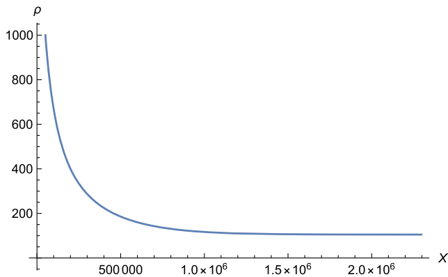
FIG. 3. The shape of a semi-infinite BIon solution for the parameters \alpha = -1 , \omega = 0.5 , g = 10^8 . The plot depicts the \mathbf{RP}^2 size of the BIon, \rho , as a function of the transverse distance X . In this particular case we used one of the critical values of c , c \simeq -10^8 - 1.21306127 . The size of the BIon funnel at X \rightarrow \infty is \rho \simeq 104.95 . To get the numerical solution we used the boundary condition X(2000) = 0 as an approximation to (4.31). Very similar solutions exist in the O3^- , where R \rightarrow 0 , \omega \rightarrow +\infty with R^4 \cosh(2\omega) are kept fixed.
