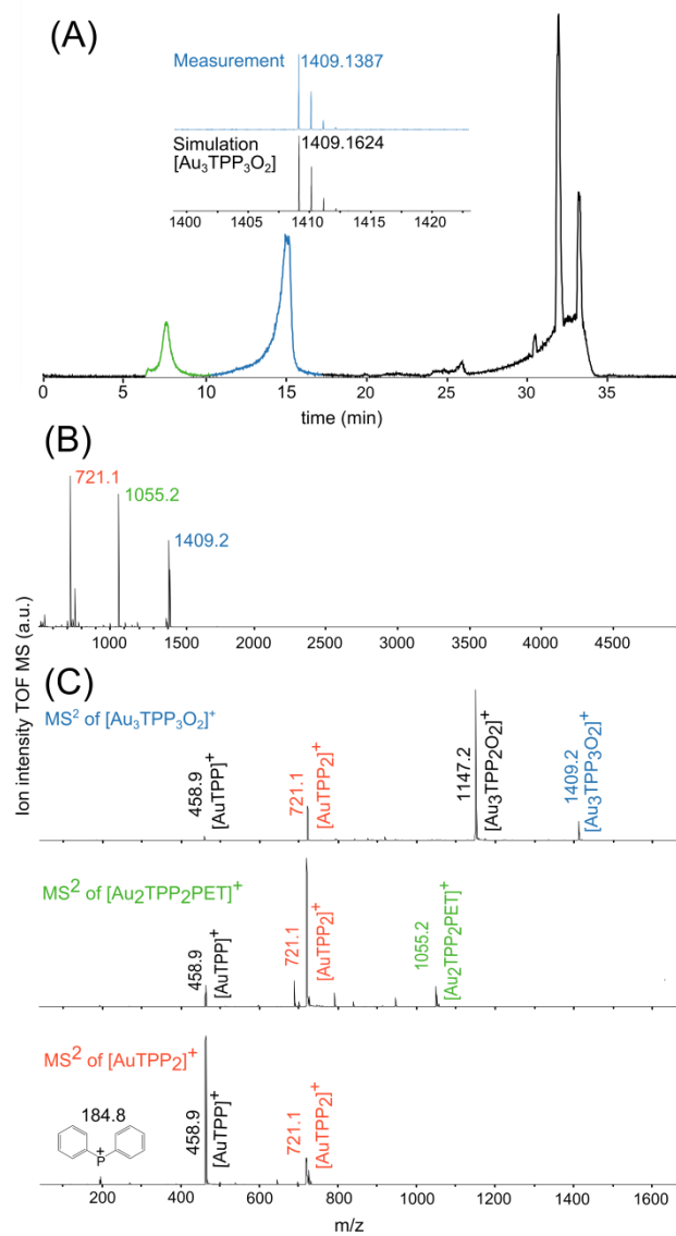
Fig. 3: MS analysis of [\text{Au}_{25}(\text{TPP})_{10}(\text{PET})_5\text{X}_2]^{2+} and contained byproducts. A) Base peak chromatogram of \text{Au}_{25} NCs measured with ESI-MS. B) MALDI-MS of \text{Au}_{25} NCs. C) MALDI-MS/MS analysis of components present in B). Same color in different figures indicates the same compound or the same fragment.
