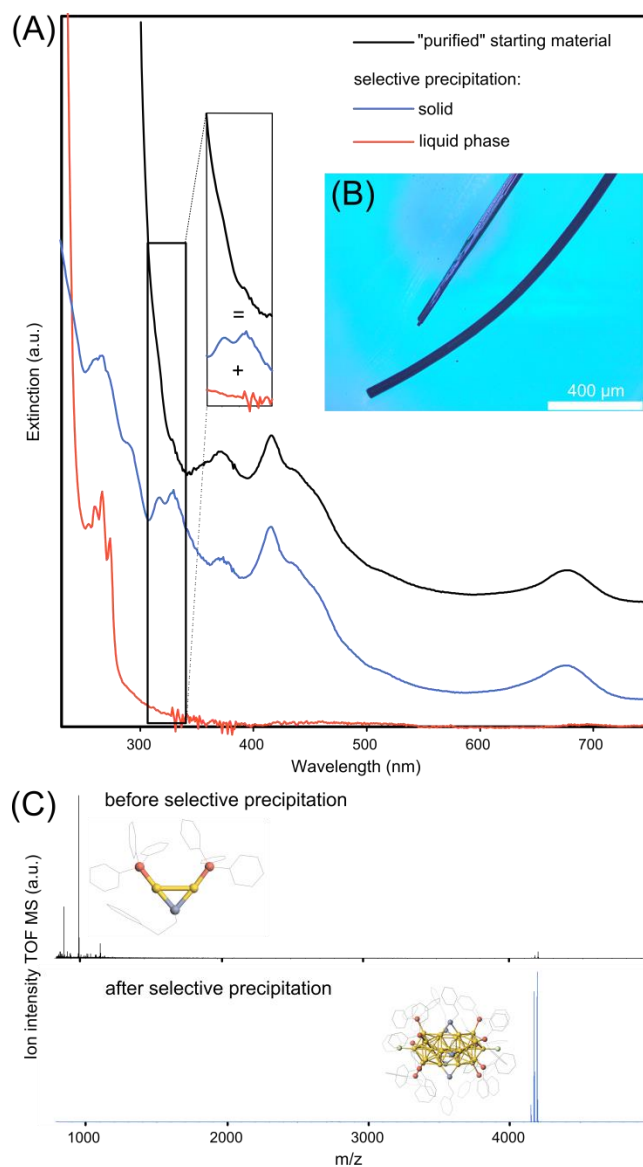
Fig. 4: A) UV-Vis spectra of the “purified” [\text{Au}_{25}(\text{TPP})_{10}(\text{PET})_5\text{X}_2]^{2+} NC suspension and from it selectively separated compounds, y -offset for a better overview. The inset illustrates the broadening of \text{Au}_{25} NCs optical features by the presence of \text{Au}_2/\text{Au}_3 complexes. B) Optical microscope image of \text{Au}_{25} NC crystals. C) ESI-MS analysis of “purified” \text{Au}_{25} NC suspension and after selective purification. The inset shows the crystal structure of the most intensive component, \text{Au}_2 complex and \text{Au}_{25} NC, respectively.
