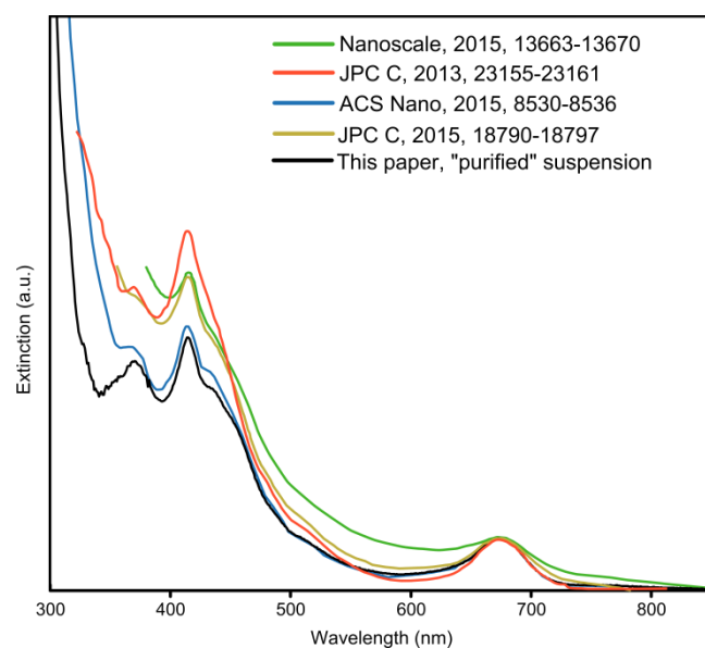
Fig. 2: Optical spectra reported for [\text{Au}_{25}(\text{TPP})_{10}(\text{PET})_5\text{X}_2]^{2+} NCs illustrating clear differences in the relative intensities of the peaks and the expression of the fine structure. All data were digitized from the cited source and normalized to 675 nm (HOMO to LUMO transition).
