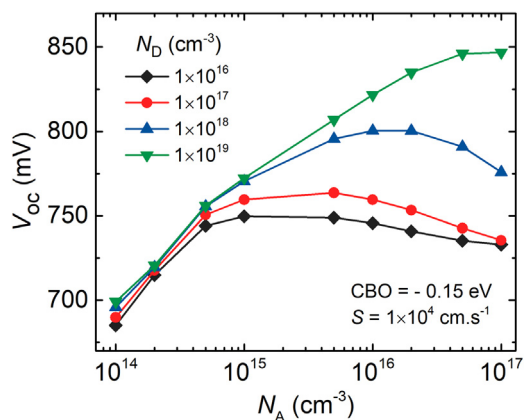
Fig. 7. V_{oc} vs. acceptor concentration ( N_A ) of the CdTe layer for varying donor concentrations ( N_D ) in the CdZnS layer, when CBO = -0.15 eV and S = 10^4 \text{cm s}^{-1} .
