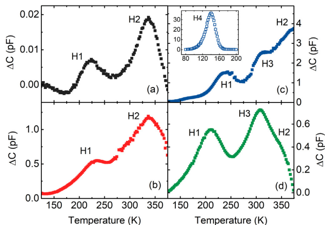
Fig. 8. DLTS spectra recorded for samples with various bulk As concentrations: (a) 1 \times 10^{16} , (b) 3 \times 10^{17} , (c) 4 \times 10^{18} , and (d) 1 \times 10^{19} \text{As cm}^{-3} . Spectra were recorded over a 125–375 K range with a 2 K increment using a pulse width of 0.1–100 ms depending on the sample. Inset to (c) shows the low temperature (80–200 K) DLTS spectrum recorded for 4 \times 10^{18} \text{As cm}^{-3} using a pulse width of 1 \mu\text{s} . Positions of observed hole (H) trap levels are labelled.
