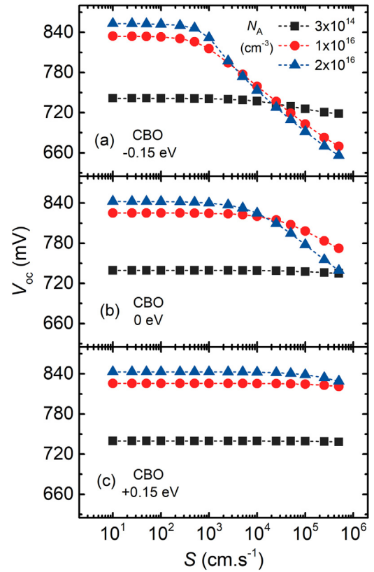
Fig. 6. V_{oc} vs. interface recombination velocity ( S ) between CdZnS and CdTe layers for varying acceptor concentration ( N_A ) and for three different conduction band offset ( \chi_{\text{CdTe}} - \chi_{\text{CdZnS}} ) values of (a) CBO = -0.15 eV, (b) CBO = 0 eV, and (c) CBO = +0.15 eV. A small positive CBO, i.e. spike, is beneficial for maintaining the V_{oc} when S \geq 10^3 - 10^4 \text{cm s}^{-1} .
