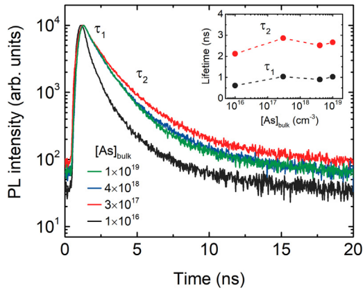
Fig. 5. PL decay curves of CdZnS/CdTe solar cells measured from the glass-side. The inset shows the extracted lifetimes, \tau_1 and \tau_2 , obtained by fitting the decay curves with two exponentials. \tau_2 is believed to represent the minority carrier lifetime in the CdTe absorber layer.
