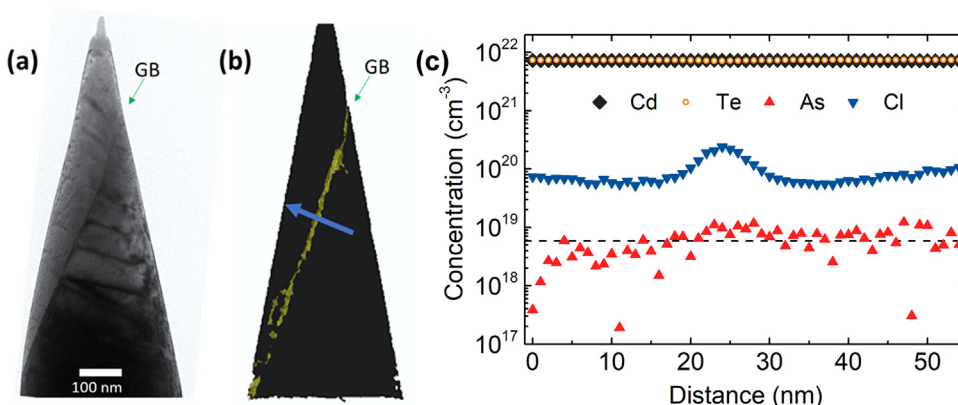
Fig. 1. A needle-shaped APT px CdTe specimen, exhibiting two grains and a GB, as imaged by TEM (a). The APT reconstruction (b) shows a 0.9 at% Cl surface (yellow) and a 97.6 at% Cd + Te surface (black), which highlights the GB location, and the region that was used for the 1-D atomic concentration profiles of elements Cd, Te, Cl, and As (c) in the direction of the blue arrow in (b), derived from APT. No As accumulation, but Cl segregation can be seen around the GB. The dashed line is the mean value of As present in the region of interest. (For interpretation of the references to color in this figure legend, the reader is referred to the web version of this article).
