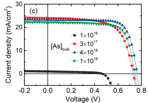
Fig. 3. (a) SIMS As concentration [As] depth profile and (b) acceptor density and activation ratio of the absorber in the CdTe:As solar cells studied. The \sim 1 \times 10^{16} As \text{cm}^{-3} sample is unintentionally-doped and does not contain the heavily-doped ( \sim 1 \times 10^{19} As \text{cm}^{-3} ) back-contact layer. (c) Typical light J-V curves of the CdTe:As solar cells.
