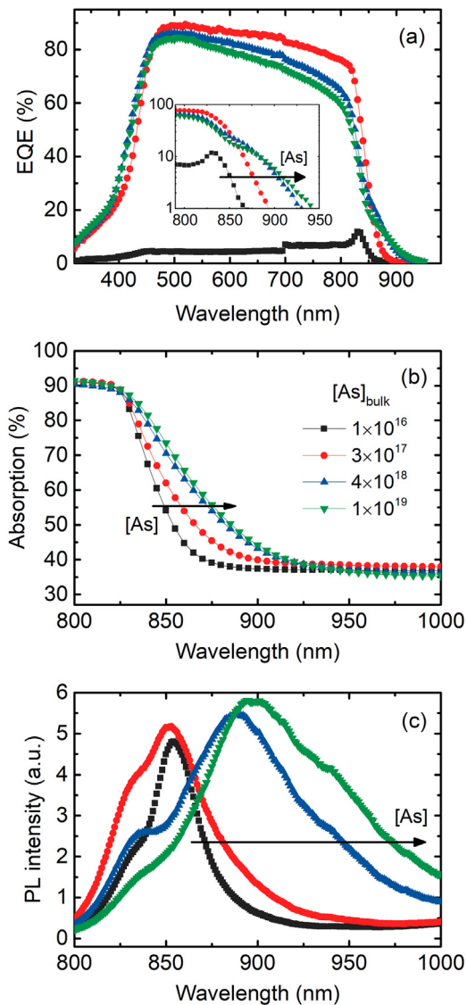
Fig. 4. (a) EQE, (b) absorption, and (c) PL (glass-side) spectra of CdTe:As solar cells as function of the As concentration in the bulk. Note the step feature at 700 nm in (a) is an artefact of lamp changeover of the EQE system.
