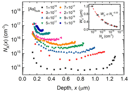
Fig. 2. Acceptor concentration ( N_A ) profile for px CdTe samples produced by in-situ doping with As concentration increasing from 1 \times 10^{16} As \text{cm}^{-3} (bottom profile) to 1 \times 10^{19} As \text{cm}^{-3} (top profile). Inset: Variation of W_D with N_A , exhibiting an inverse relationship; W_D \propto N_A^{-0.33} .
