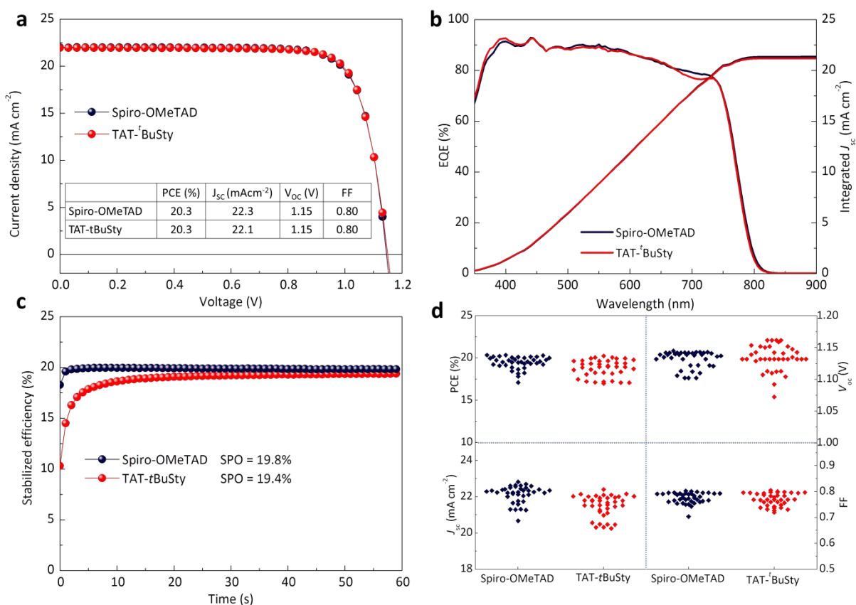
Figure 4. Device performance using Spiro-OMeTAD and TAT- t BuSty as HTM layers. (a) J - V characteristics of optimized perovskite solar cells with FTO/SnO 2 /perovskite/HTM/Au device structure. (b) External quantum efficiency (EQE) spectra. (c) Stabilized power output (SPO) of the champion cells, determined by holding the cell at a fixed voltage near the maximum power point on the J - V curve for 60 s. (d) Distribution of PCE, V_{oc} , J_{sc} and FF for devices tested in this work.
