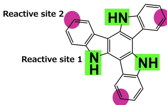
Figure 1. Triazatruxene (TAT) molecular structure with reactive sites highlighted.
