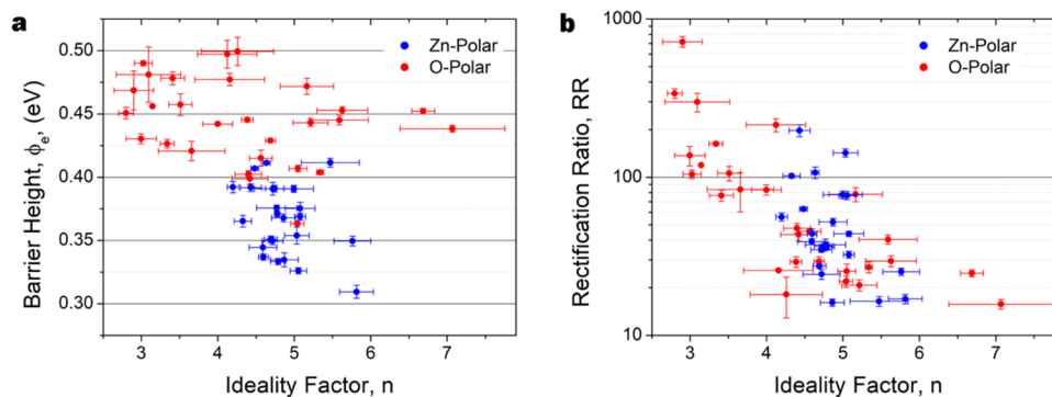
Figure 2. (a) Graph showing the relationship between ideality factor, n , and effective barrier potential height, \phi_e , for measured nanorods on the Zn-polar and O-polar samples after the oxygen plasma treatment. (b) Graph showing the rectification ratio of Zn-polar and O-polar nanorods with Au contacts plotted against the ideality factor.
