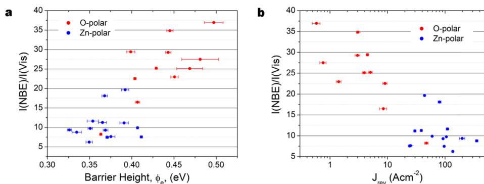
Figure 5. Graphs comparing the CL data for both samples with properties of the Au–ZnO contacts. (a) Intensity ratio of the NBE emission and visible band ( I_R ) against barrier height ( \phi_e ); (b) intensity ratio of the NBE emission and visible band ( I_R ) against the current density at -2 V ( J_{\text{rev}} ).
