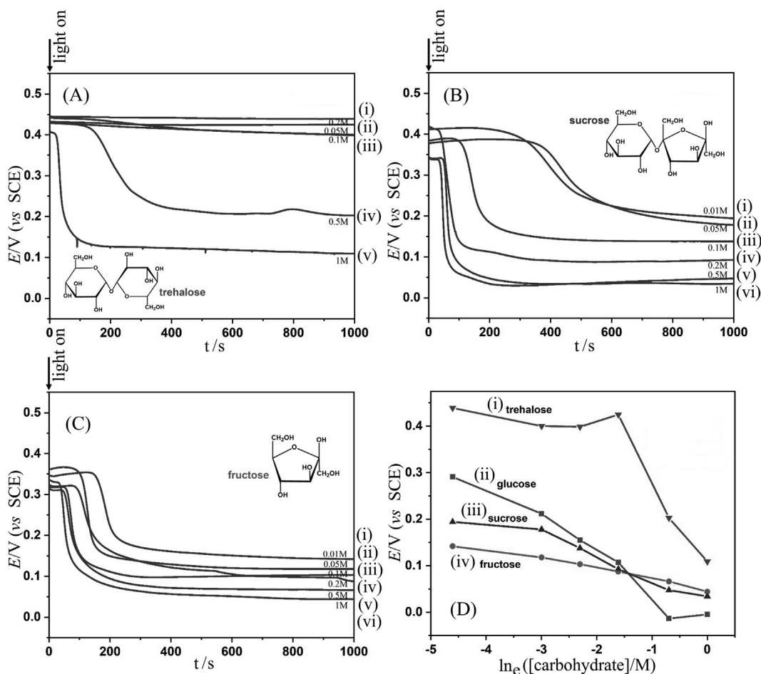
Fig. 4. (A) Chronopotentiometry (zero current) data obtained with 60 \mu\text{g} Pt@g-C 3 N 4 and 12 \mu\text{g} PIM-1 at a palladium membrane for (i) 0.05, (ii) 0.1, (iii) 0.2, (iv) 0.5, and (v) 1 M trehalose in water. (B) As above but for sucrose. (C) As above but for fructose. (D) Plot of the final equilibrium potential (at 1000 s) versus carbohydrate concentration in water for (i) trehalose, (ii) glucose, (iii) sucrose, and (iv) fructose.
