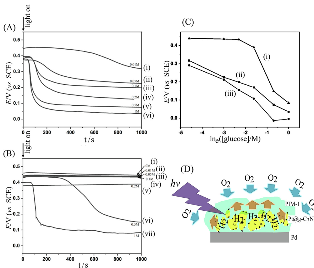
Fig. 3. (A) Chronopotentiometry (zero current) with 60 \mu\text{g Pt@g-C}_3\text{N}_4 and 24 \mu\text{g PIM-1} on palladium in (i) 0.01, (ii) 0.05, (iii) 0.1, (iv) 0.2, (v) 0.5, and (vi) 1 M glucose in water. (B) As before but for only 60 \mu\text{g Pt@g-C}_3\text{N}_4 and no PIM-1. (C) Summary plot of end potential (at 1000 s) as a function of glucose concentration in water for (i) no PIM-1, (ii) 24 \mu\text{g PIM-1} , and (iii) 12 \mu\text{g PIM-1} . (D) Schematic drawing of the photocatalytic hydrogen production under a PIM-1 film competing with oxygen ingress.
