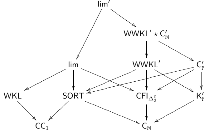
FIGURE 2. Location of \text{CFI}_{\Delta_2^0} in the Weihrauch lattice. An arrow from P to Q represents the reduction Q \leq_W P . No additional arrows can be added other than those that follow by transitivity. For (non-)reductions not explicitly mentioned above, see [6, Sections 4 and 5 and Figure 5].
