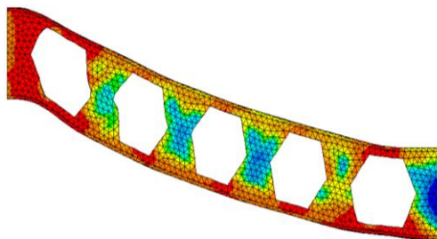
c) Hexagonal castellated steel beam
