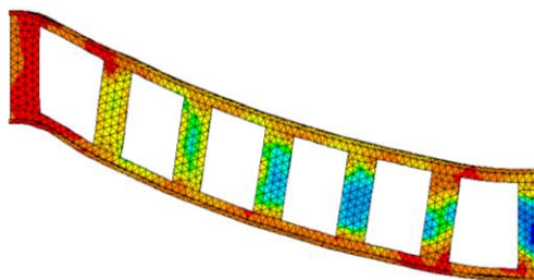
d) Rectangular castellated steel beam
