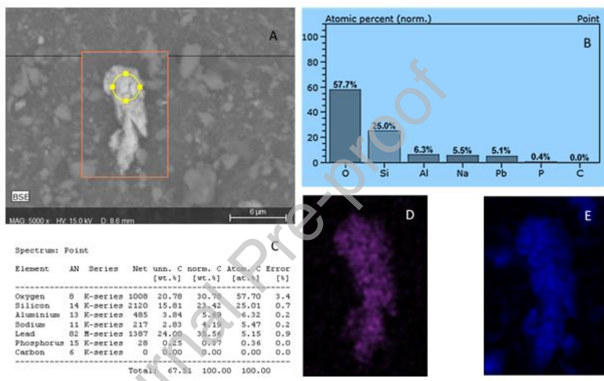
Figure 5. Is an example of EDX data referring to the composition of a grain particle found in face mask 4 (paw patrol). (A) is the image generated by the SEM at x5000, (B) shows the EDX data plotted graphically, whilst C is tabulated elemental composition data. Image D is false colour map for elemental lead (Purple) and image E (blue) is an elemental map of Si the same grain.
