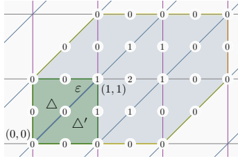
FIGURE 8. Bernstein coefficients of the box spline 2\mathcal{B}_{(2,1,1)} .
