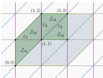
FIGURE 2. Multicell domain M = \cup_{i=1}^4 \hat{\Delta}_i , with edges \varepsilon_i = \bar{\Delta}_i \cap \bar{\Delta}_{i+1} for i = 1, 2, 3 .
