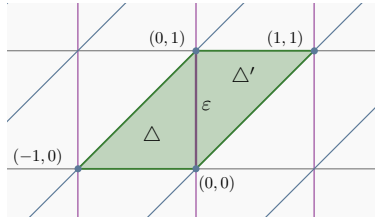
FIGURE 7. The triangles \Delta and \Delta' in G define the multicell domain M in Example 23, the triangles share the edge \varepsilon \in E_2 that is parallel to the directional vector \mathbf{e}_2 .
