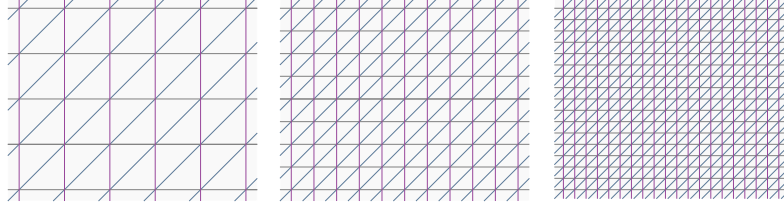
FIGURE 9. Three levels of three-directional hierarchical grids.
