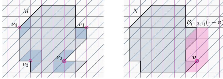
FIGURE 4. On the left, the shadowed regions around the vertices \nu_i \in M correspond to the triangles in \text{star}(\nu_i) \cap M , respectively; notice that in this multicell domain M , by Definition 11, the only over-concave vertex is \nu_2 . On the right, the multicell domain N does not have over-concave vertices; the figure also illustrates Definition 25 from Section 4, the shadowed region corresponds to the support of the box spline \mathcal{B}_{(1,3,1)}(\cdot - \mathbf{v}) considered in Example 26.
