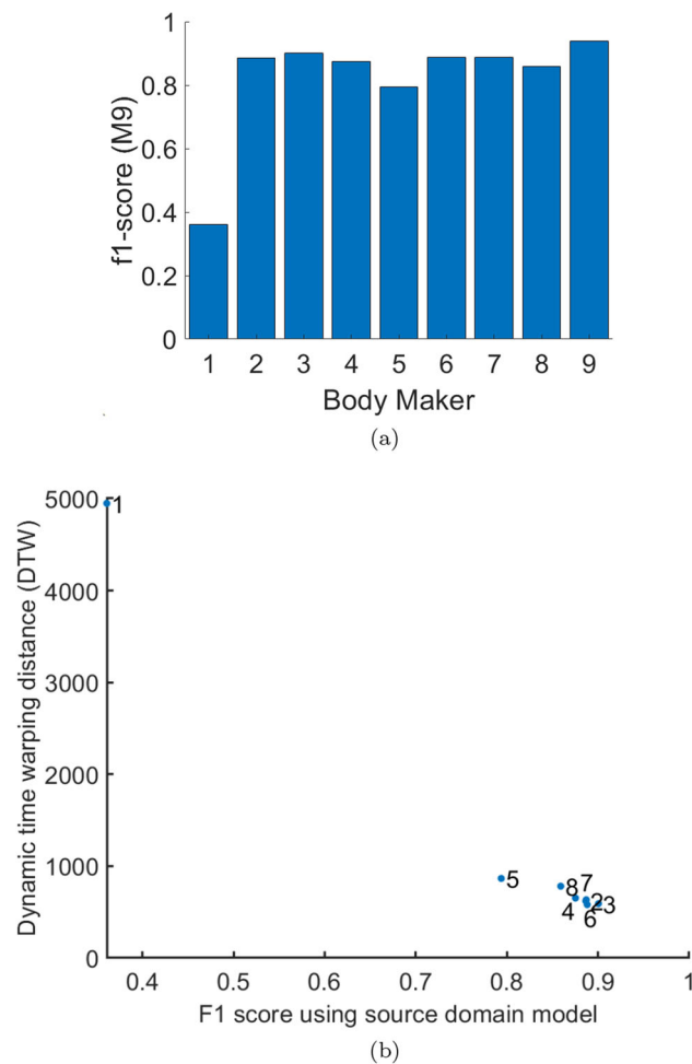
Fig. 6 Evaluation of predictive performance using source model, \mathcal{M}_9 , to predict on target datasets. a Comparative evaluation of F-score obtained by using the source model, \mathcal{M}_9 , to predict on the target datasets. b Scatter plot showing relationship between F-score and DTW distance
