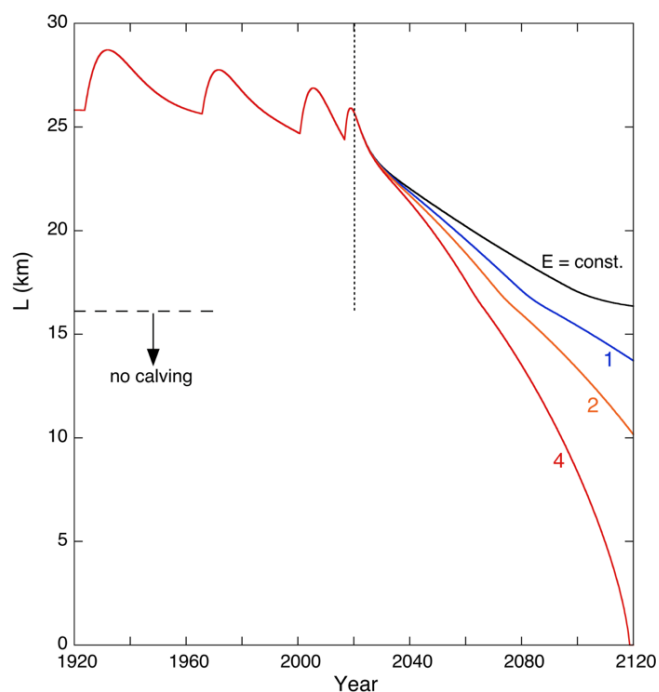
Figure 9. Glacier length L for different climate change experiments. The black curve refers to a calculation in which E is kept constant at its 2000–2019 mean value. The colour labels refer to the imposed constant rate of change in E per year from 2020 onwards.
