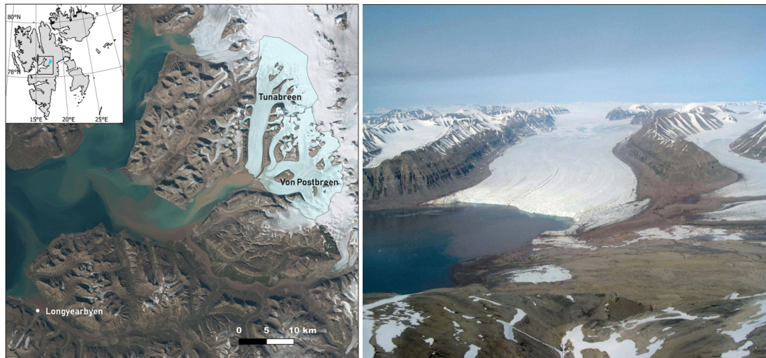
Figure 1. Left: location of Tunabreen and Von Postbreen in Svalbard (inset). Background image is from a 2020 Sentinel-2 mosaic ( https://toposvalbard.npolar.no , last access: 24 May 2022). Right: photograph of Tunabreen in 2015 (© Anders Skoglund, Norwegian Polar Institute).
