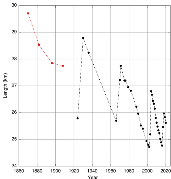
Figure 2. Length of Tunabreen from historical documents, aerial photographs, and satellite images (Flink et al., 2015, with additions). The first four data points in red refer to the period that Tunabreen and Von Postbreen formed a joined front.
