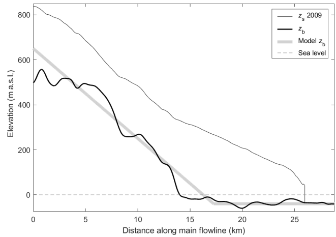
Figure 4. Cross-section along centreline profile (shown in Fig. 3) of the main flow band, with band averages of surface topography (thin black line) from the 2009/2011 NPI DEM and bed topography from the Fürst et al. (2018) reconstruction (0–12.5 km), 2015 helicopter radar measurements (12.5–25 km), and hydrographic data in the fjord (Norwegian Mapping Authority Hydrographic Service). A piecewise linear profile is fit to the bed profile for the MGM.
