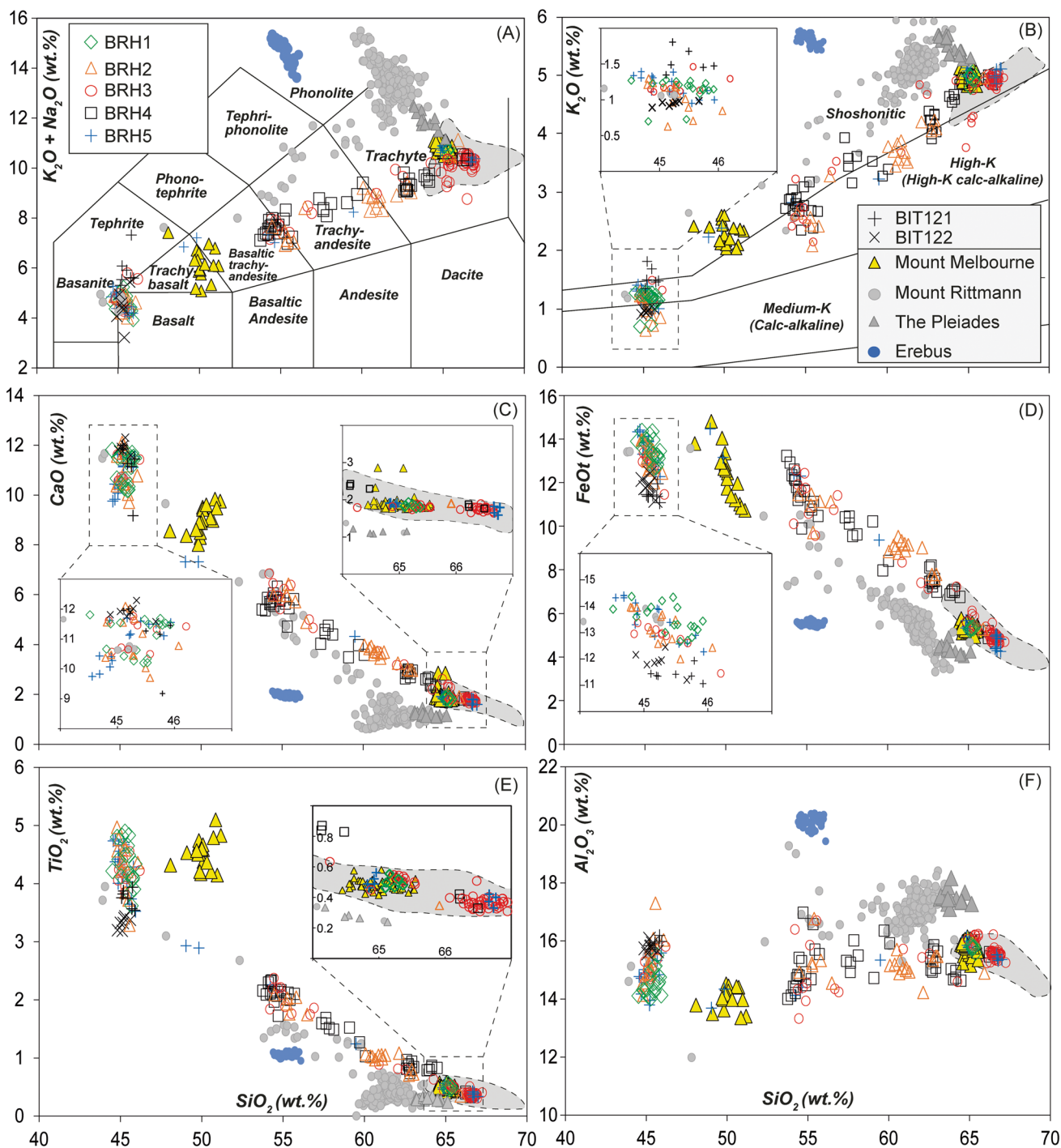
Fig. 5 Bivariate major elements plots depicting the significant volcanic glass heterogeneity of the BRH1 to 5 tephra deposits which range from basalts through to trachytes. (A) Total alkalis vs. silica classification diagram (TAS) following LeBas et al. (1986); (B) K_2O vs. SiO_2 following Peccerillo and Taylor (1976). The trachytic glasses of the BRH 1 to 5 tephra layers plot along the same evolution trend as those previously analyzed from Mount Melbourne (Del Carlo et al.
