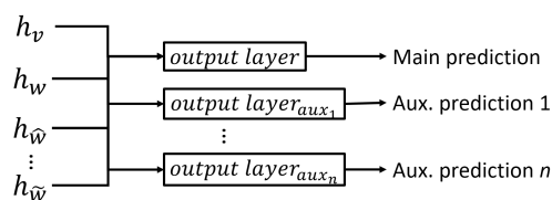
Figure 4: Illustration of multi-task learning for relating learnt features to relevant physical quantities.
