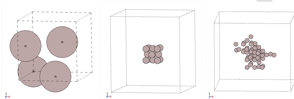
Figure 5: FCC Bravais crystal lattice (left) and growing crystal structures (centre: seed, right: intermediate).
