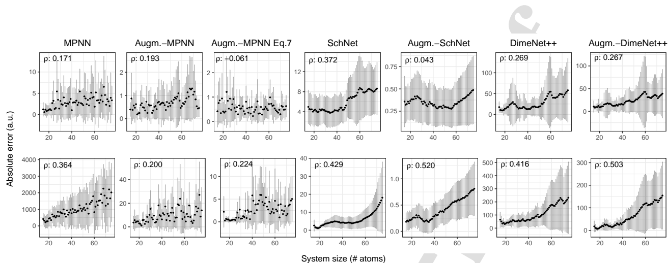
Figure 9: Impact of system size on accuracy when trained on systems of up to 75 (top) and 25 (bottom) atoms from UCG.
