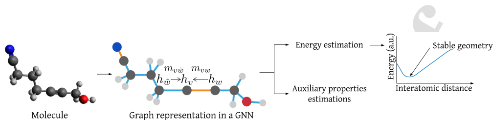
Figure 1: Graph representation of a molecule (from QM9) for GNN estimation of potential energy and stable geometry. Nodes of states \mathbf{h}_i are atoms and colour denotes atom type (black: carbon, white: hydrogen, blue: nitrogen, red: oxygen). Edges link chemically bonded atoms and colour denotes bond type (blue: single bond, orange: double bond). Non-bonded atoms may also share edges in fully connected graphs, but these edges are not represented for readability. Messages \mathbf{m}_{ij} are exchanged across edges. The GNN outputs an energy estimate, along with the estimates of one or several auxiliary (physical and chemical) properties in the case of multi-task learning. Energy estimates at different molecule geometries may be used to identify stable configurations at the minimum of energy. Left drawing is from (Glavatskikh et al., 2019).
