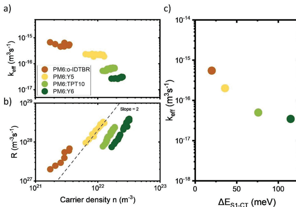
Figure 6. a) Effective bimolecular recombination rate coefficient k_{\text{eff}} and b) recombination rate R versus carrier density, and c) k_{\text{eff}} against \Delta E_{S_1-CT} for PM6:o-IDTBR, PM6:Y5, PM6:TPT10, and PM6:Y6. The dashed line in (b) represents the slope of 2. The data for PM6:Y6 are taken from previous work from our group. [44]
