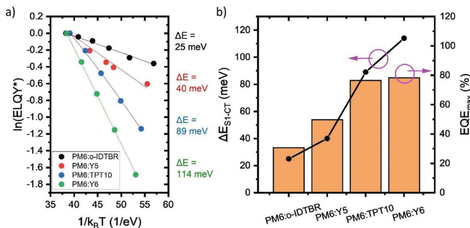
Figure 2. a) Temperature-dependent ELQY of the devices, the temperature-dependent ELQY values of PM6:Y6 are taken from a previous paper from our group, [14] and refitted with Equation (1). b) The fitted \Delta E_{S_1-CT} values and EQE amplitude of each system.
