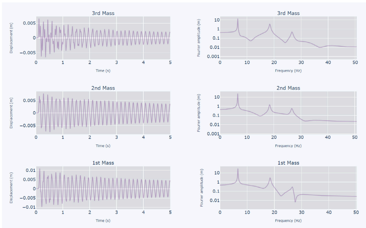
Fig. 6. Outputs from the hammer testing data simulator tool. On the left an example of the displacement time-histories of each of the three masses is shown, and on the right the corresponding Fourier amplitude for each mass. The hammer tool is simulated with zero initial conditions and with the hammer hitting first mass at time t = 0.1 s with a force intensity of F = 300 N.
