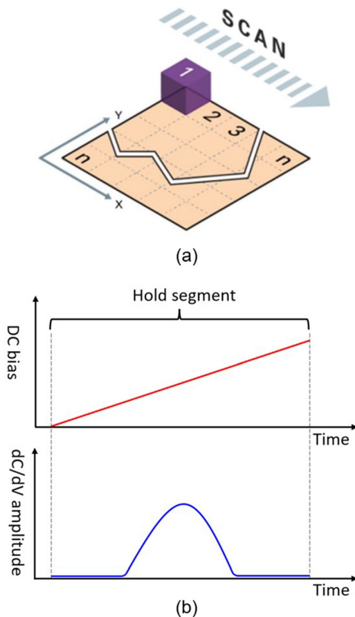
FIG. 1. The working principle of hyperspectral SCM: (a) schematic of scan pattern during the acquisition of hyperspectral SCM data. 12 Reproduced with permission from De Wolf et al. , Microsc. Today 26 (6), 18–27 (2018). Copyright 2018 Microscopy Society of America. (b) Patterns of the input dc bias (red) and the corresponding output dC/dV amplitude (blue) in the hold segment.
