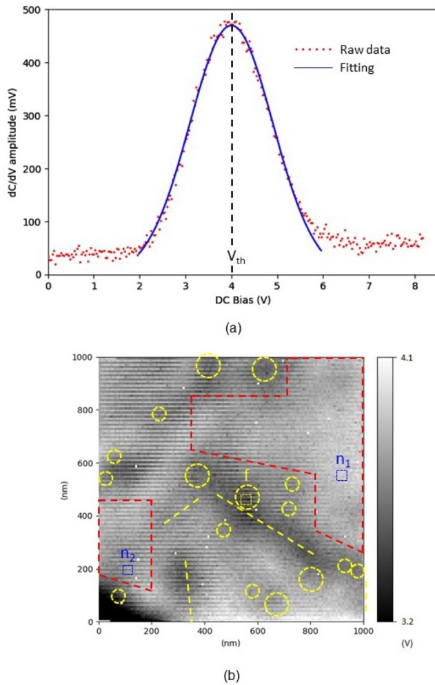
FIG. 5. (a) Determination of local V_{th} value by fitting the raw data of a local dC/dV - V spectrum captured in hyperspectral SCM mode. Local V_{th} value is defined as the peak position. (b) V_{th} distribution of the same area in Fig. 2 after fitting each dC/dV - V spectrum at each pixel. Fissures are highlighted in yellow. The V_{th} variation in non-fissure regions is highlighted in red. A fissure (f) and two non-fissure regions ( n_1 and n_2 ) are labeled.
