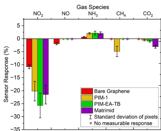
Figure 9. Bar chart comparing the selectivity of bare graphene, PIM-1, PIM-EA-TB, and Matrimid-coated 3 \times 3 graphene pixel array sensors exposed to various gases: 5 ppm nitrogen dioxide ( \text{NO}_2 ), 5 ppm ammonia ( \text{NH}_3 ), 5 ppm nitric oxide ( \text{NO} ), 100 ppm methane ( \text{CH}_4 ), and 450 ppm carbon dioxide ( \text{CO}_2 ).
